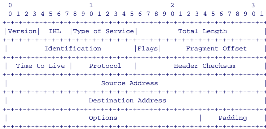
Example Internet Datagram Header
